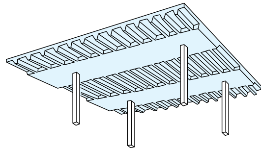
Troughed slabs (or ribbed slabs with integral beams)
